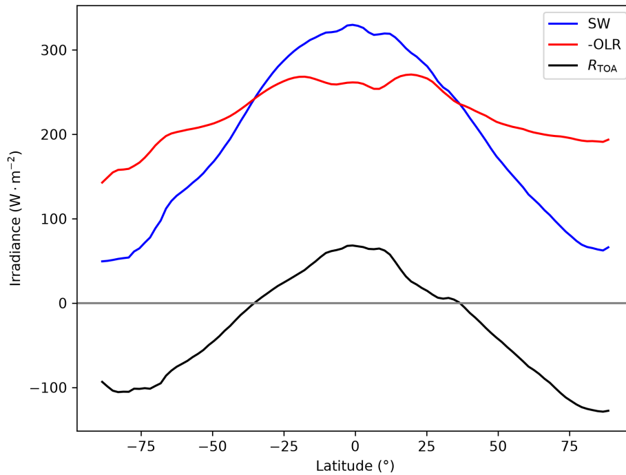
Figure 2.4: Zonal and annual mean average of irradiance from PI control simulations.
