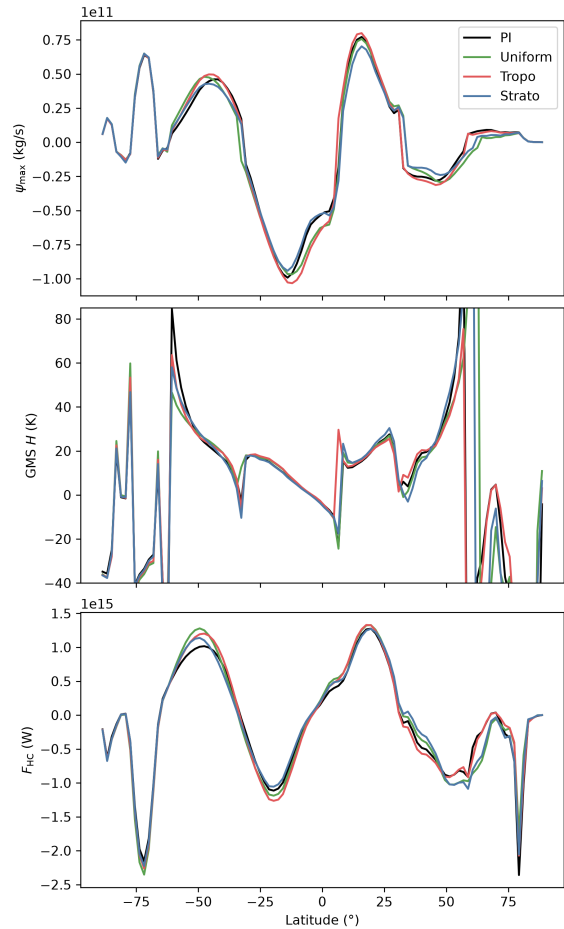
Figure 2.5: TODO: Only include PI values, increase axis labels
