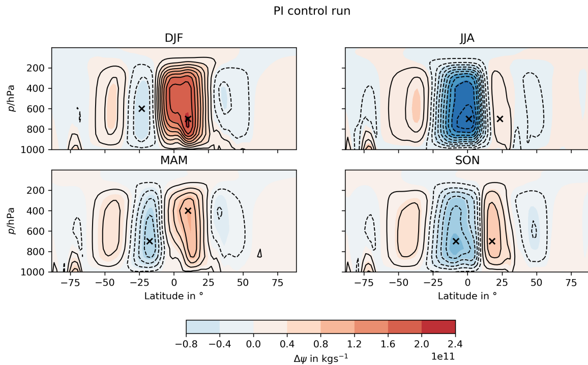
Figure 2.1: TODO: use correct PI control simulations and add annual mean while removing double equinox
