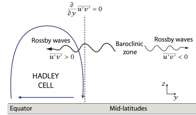
Figure 2.3: The eddy driven HC, from (Vallis, 2017)
