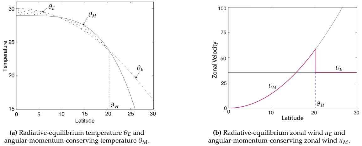
Figure 2.2: Latitudinal profiles of temperature and zonal wind under radiative equilibrium and under angular momentum conservation of the axisymmetric model, from Vallis (2017).
