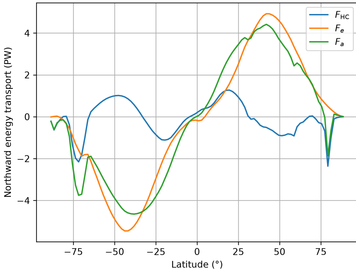
Figure 2.6: Northward energy transport
