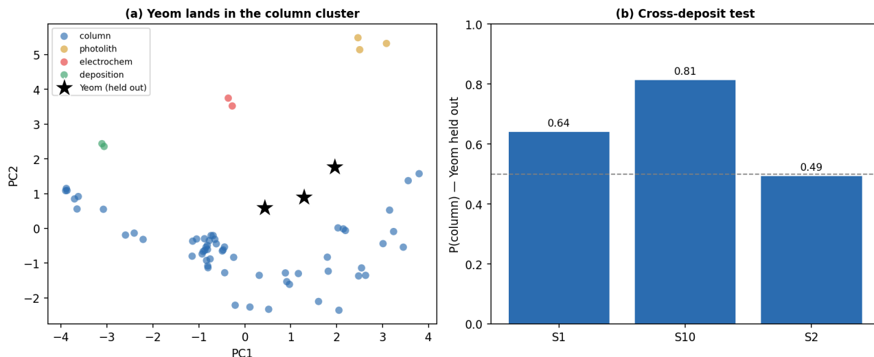
Figure 2: Cross-deposit check on an independent column deposit (Yeom SHIFT). (a) Principal-component projection of the 16-feature atlas; the held-out Yeom rotations (stars) fall in the column cluster. (b) Held-out probability of a column call for each Yeom rotation, from a classifier trained on the other deposits only.
