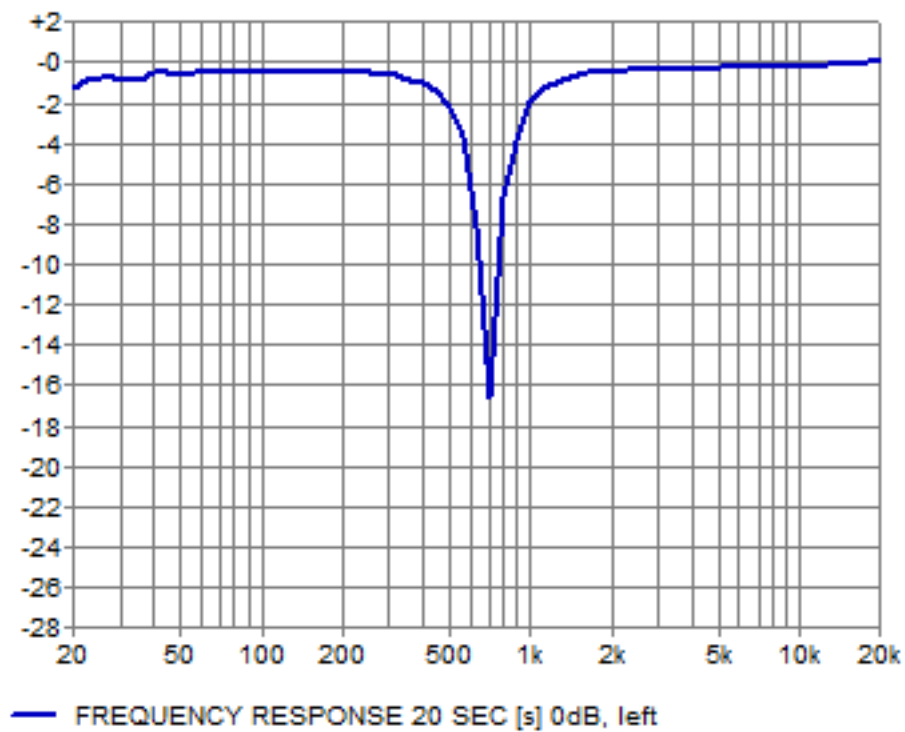
700Hz Cut
