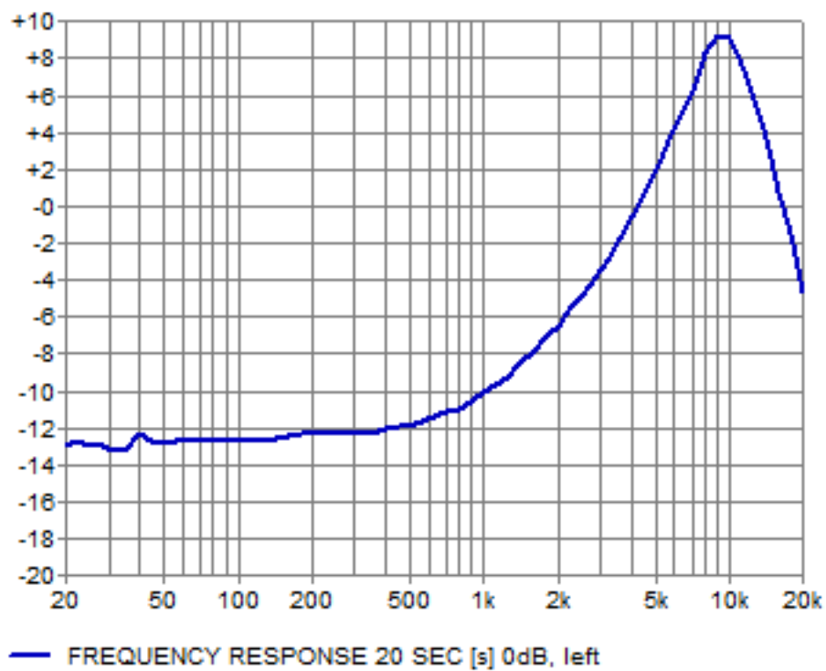
10KHz High Q
