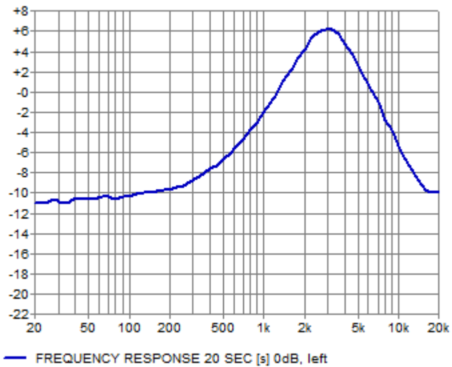
3KHz Boost
