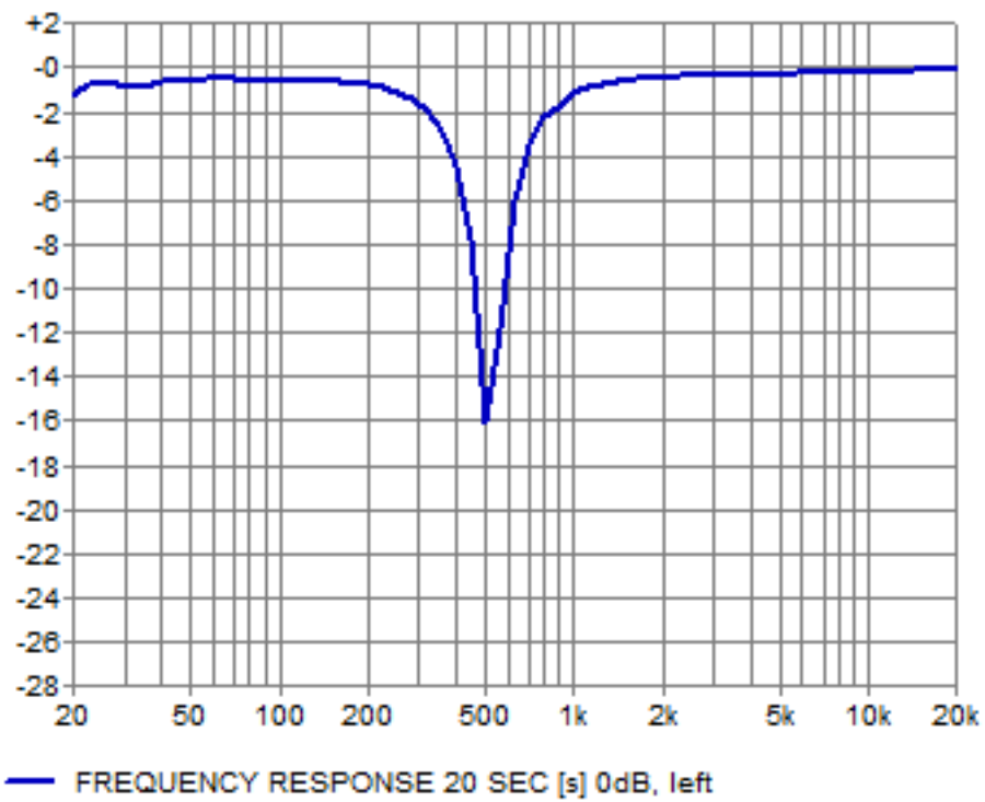
500Hz Cut
