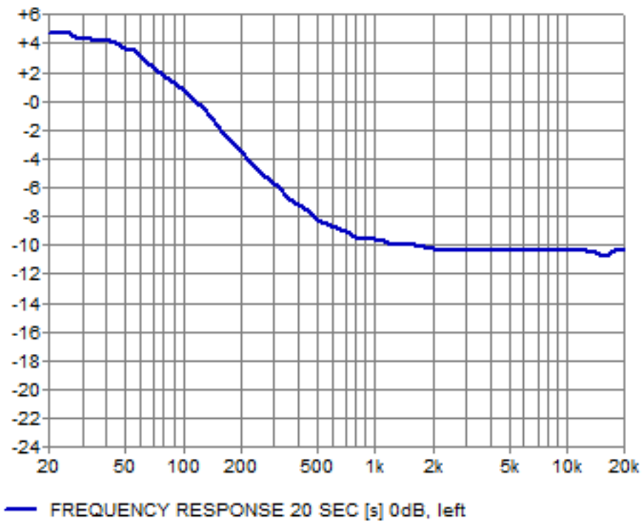
60Hz Boost
