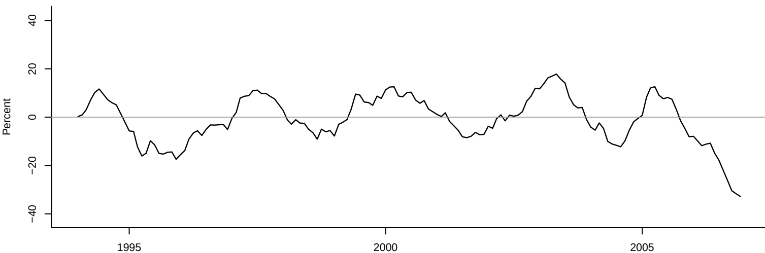
Cumulative Effect of Oil Supply Shock on Real Price of Crude Oil (Russian Model v1)
