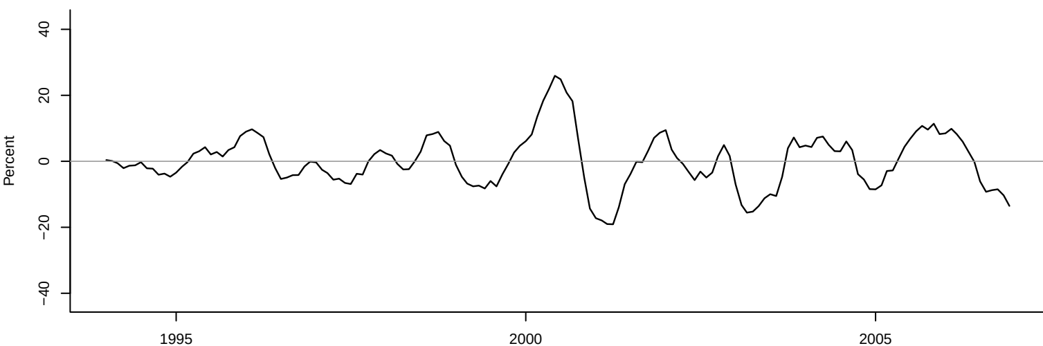
Cumulative Effect of Aggregate Demand Shock on Real Price of Crude Oil (Russian Model v1)
