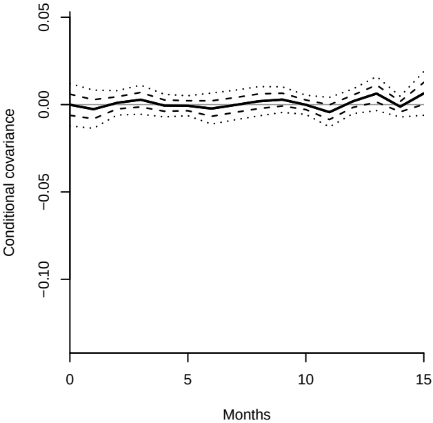
Oil supply shock
