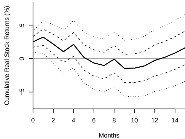
Oil-specific demand shock
