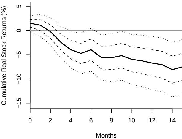
Oil supply shock
