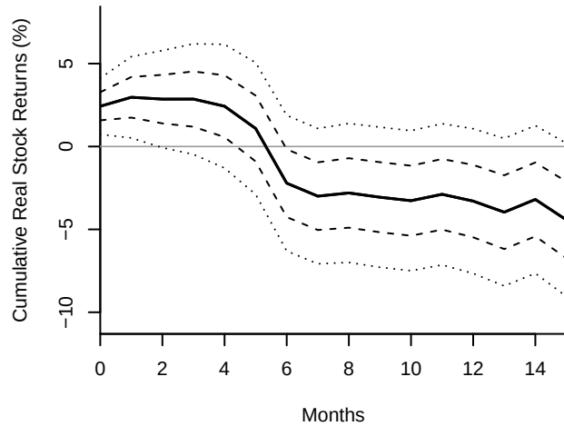
Aggregate demand shock
