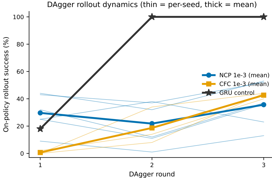
Figure 2: DAgger rollout dynamics per round. On-policy rollout success across DAgger rounds r1 \rightarrow r2 \rightarrow r3 . The GRU control climbs 18 \rightarrow 100 \rightarrow 100 ; CfC arms stay low or flat, illustrating that the aggregate does not close for the continuous-time cores (thin: per-seed; thick: per-leg mean).
