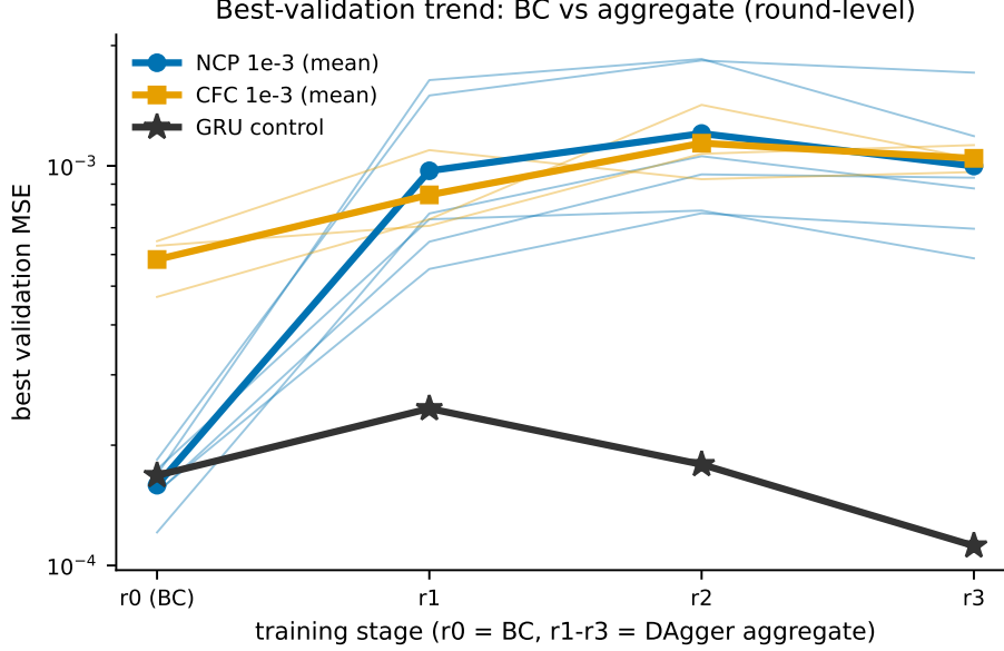
Figure 3: Best-validation trend, BC vs. aggregate. Best validation MSE per stage ( r_0 = \text{BC} \rightarrow r_1\text{--}r_3 = \text{Dagger aggregate} ) for the CfC arms (rising after aggregation, best epoch moving earlier) against the GRU control (monotonically low). Round-level (four points per cycle); full per-epoch curves are not persisted and would require re-measurement.
