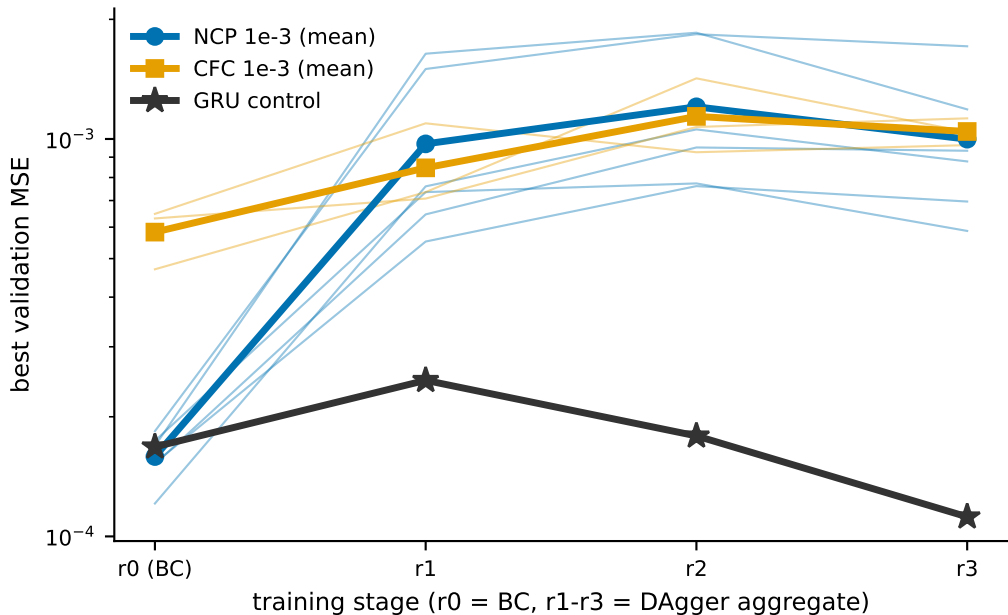
Best-validation trend: BC vs aggregate (round-level)
