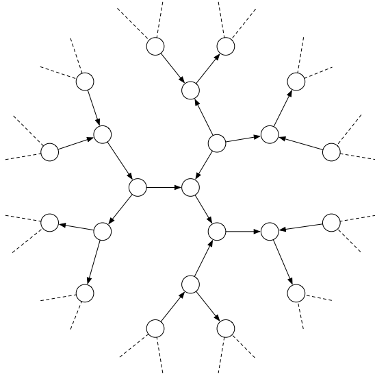
(a) A solution of sinkless orientation.
