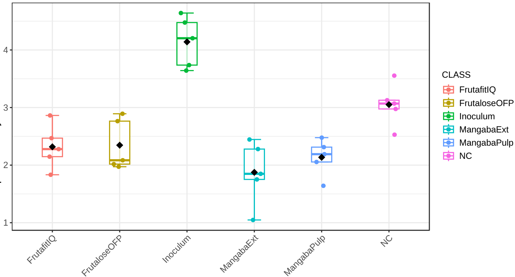
Alpha-diversity Index: Shannon
