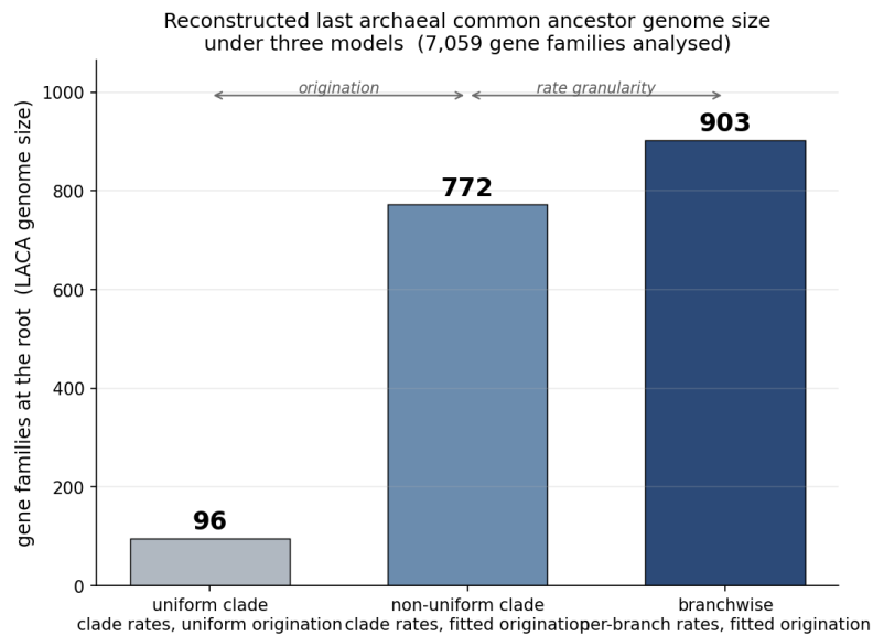
Figure 3: Reconstructed LACA genome size under three models, isolating the two effects. Uniform origination places only 96 families at the root; fitting origination with the same clade-grouped rates raises it to 772 (the origination effect), and the branch-wise rates add a further 131 to 903 (the rate-granularity effect). Origination dominates, rate granularity refines. (Of 7,059 families.)
