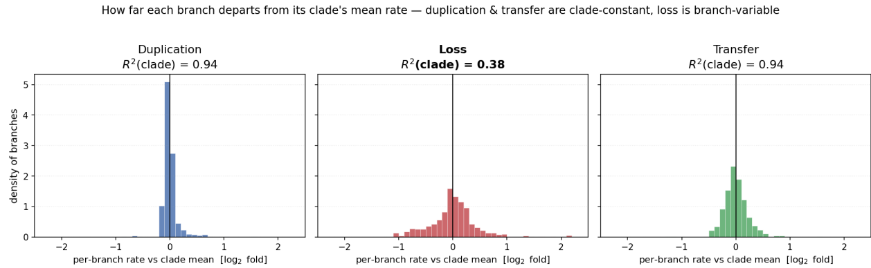
Figure 2: Departure of each branch's fitted rate from its clade's mean rate (log 2 fold; shared axes). Duplication and transfer form a sharp spike at zero — the per-branch estimates scarcely leave their clade mean, so clade membership explains R^2 \approx 0.94 of the variance — whereas loss is broad ( R^2 \approx 0.38 ), i.e. branch-specific. Gene gain (duplication, transfer) is well summarised by one rate per clade; gene loss is not.
