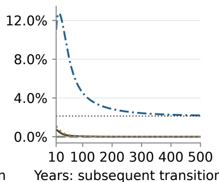
C. Capital g_K - (n + \gamma)
