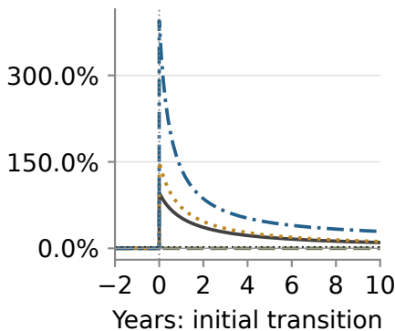
B. AI services g_X - (n + \gamma)
