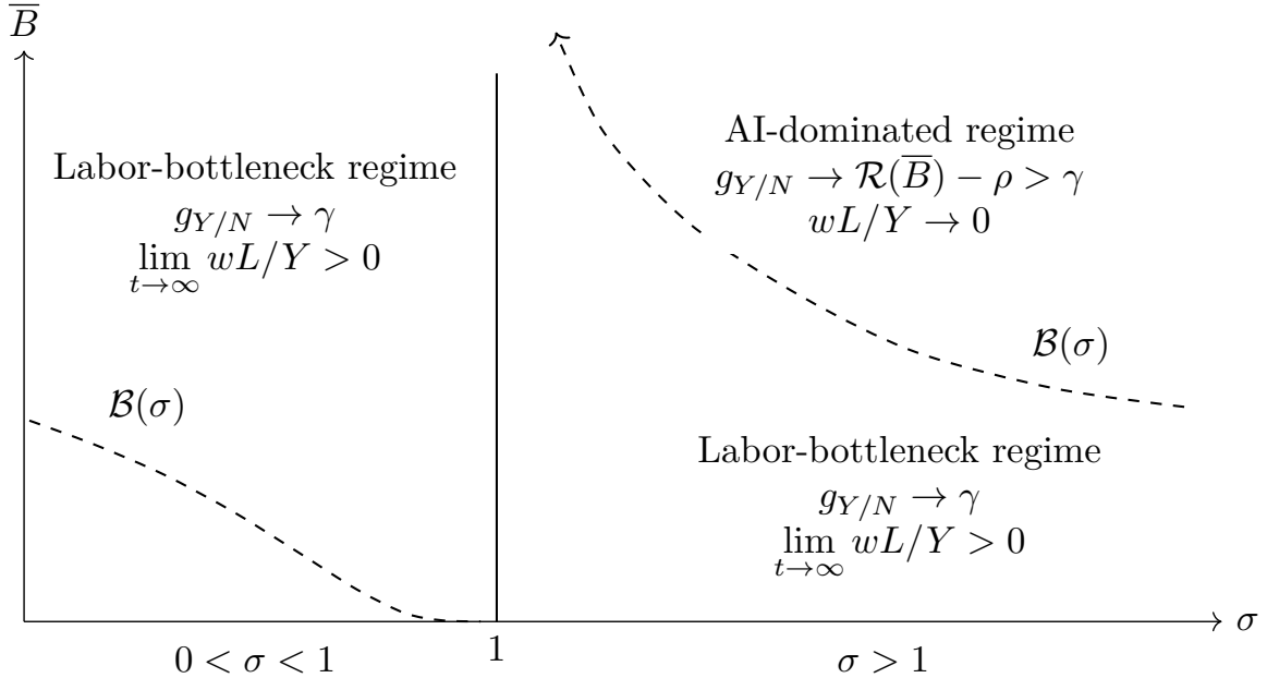
Figure 3: Constructed regimes with a finite upper bound. The vertical axis is linear and the curves are schematic rather than calibrated. For 0 < \sigma < 1 , \overline{B} > \mathcal{B}(\sigma) is the condition for the positive-labor-share construction in Proposition 1(i). For \sigma > 1 , the curve separates the labor-bottleneck and AI-dominated equilibria in Proposition 1(iii) and 1(iv).
