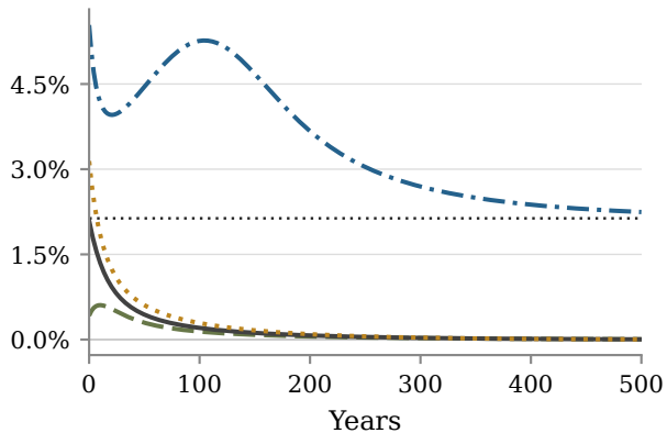
B. Capital per effective labor g_K - (n + \gamma)
