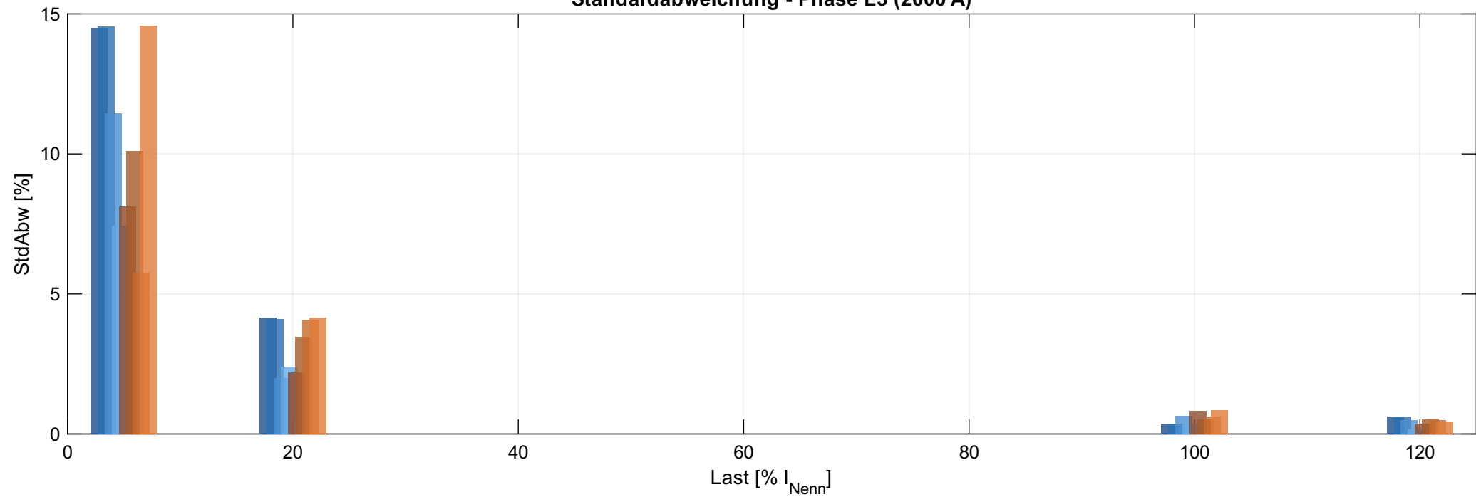
Standardabweichung - Phase L3 (2000 A)
