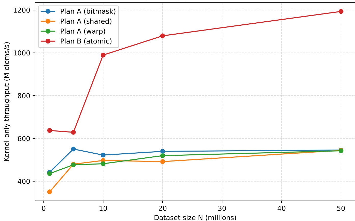
Q5: Kernel-only Throughput vs N — hit=0.50, uniform
