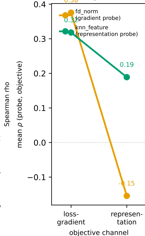
(B) which probe wins by channel
