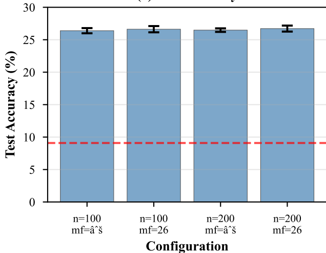
(a) Test Accuracy
