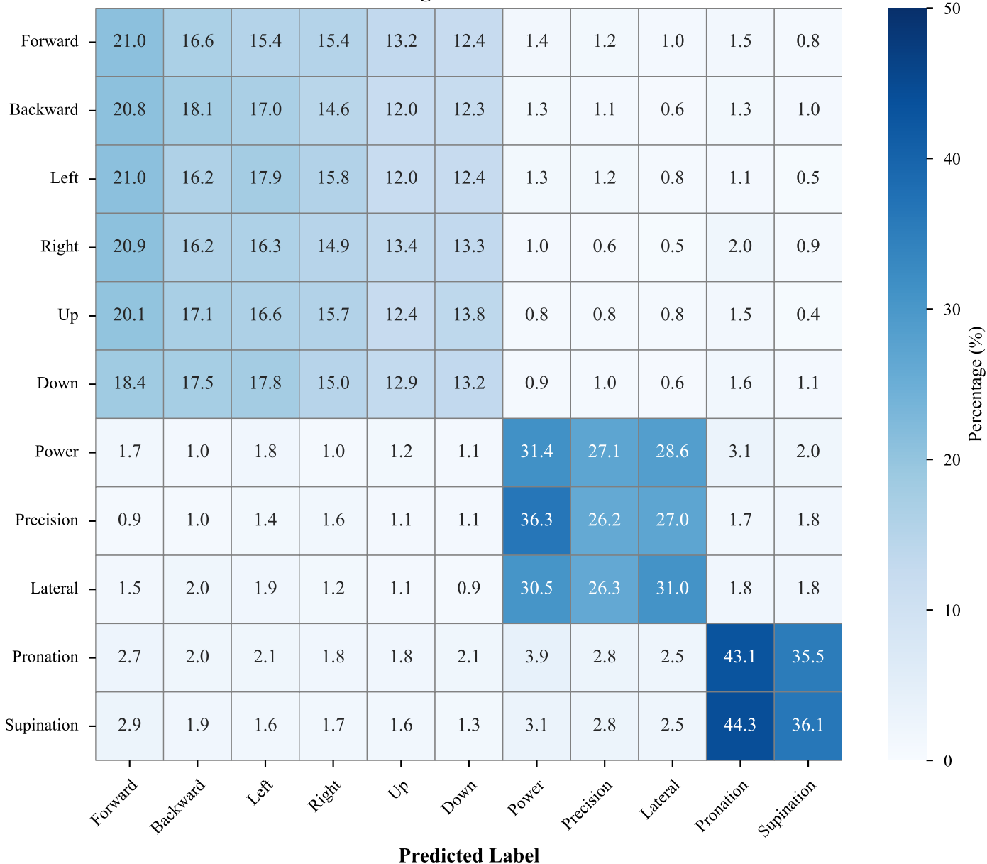
SVM Confusion Matrix (C=100, \hat{I}^3=0.01 ) Averaged over 5 trials
