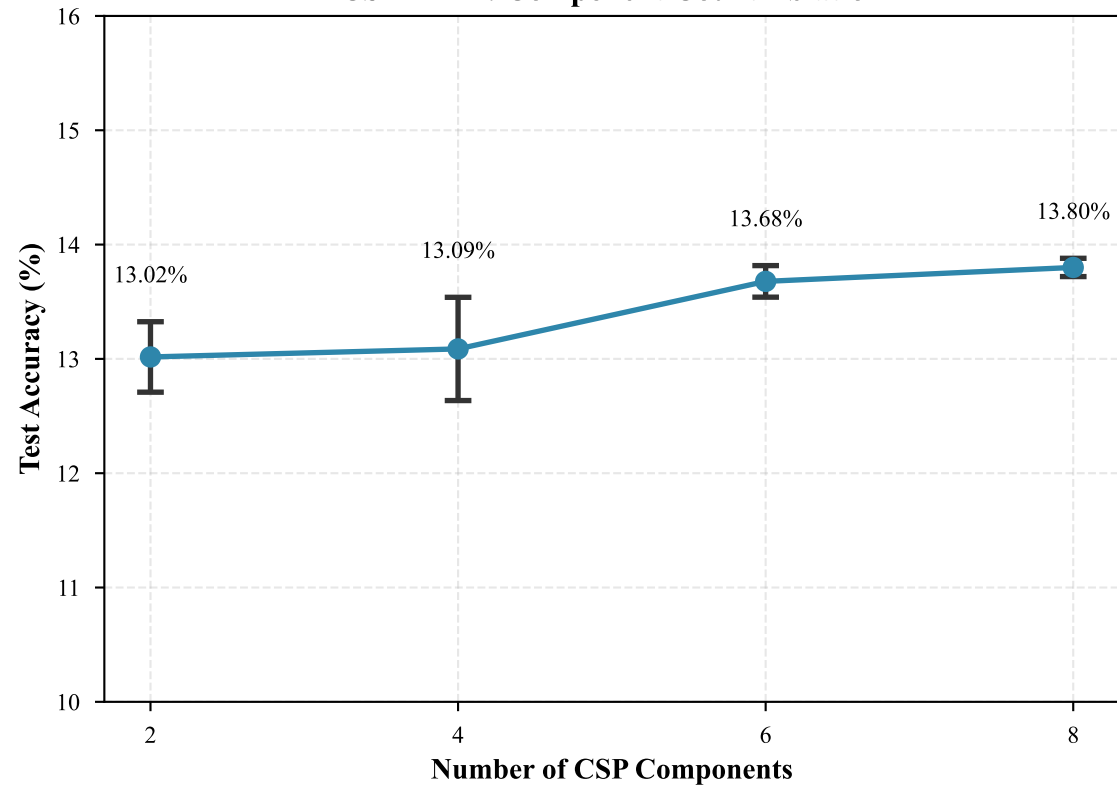
CSP+LDA: Component Count Ablation
