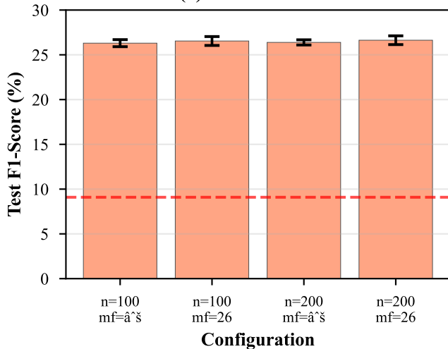
(b) Macro F1-Score
