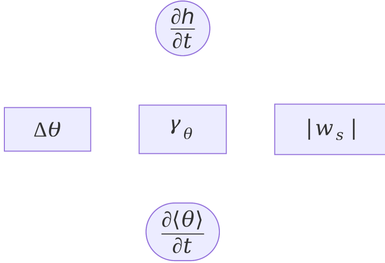
Figure 1.4: Feedback diagram illustrating the effect of large-scale forcing conditions on the evolution of the ABL. In squares, forcing parameters; in round shapes, time derivatives of key state variables.
