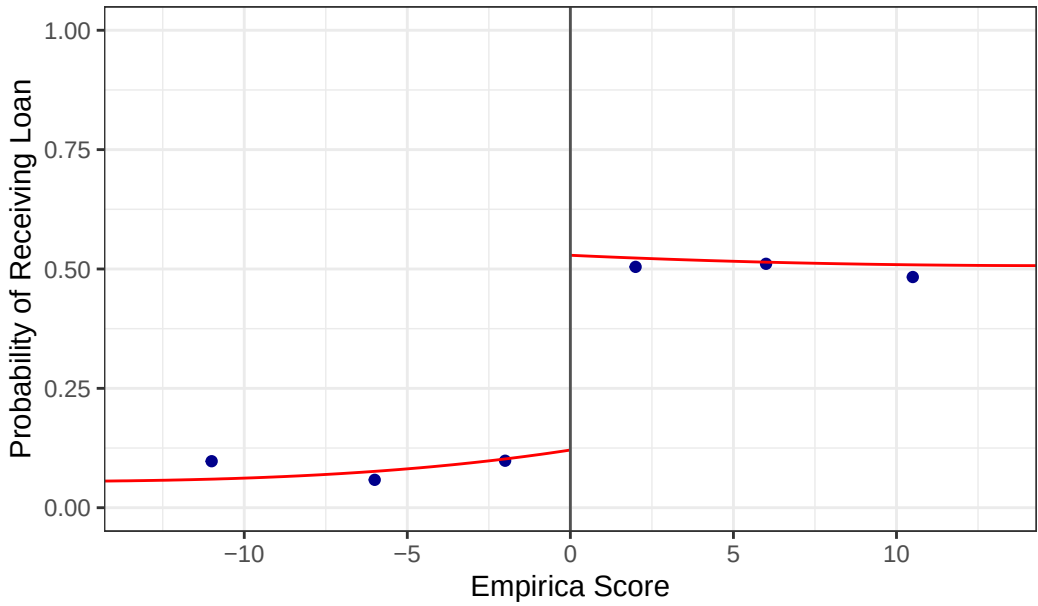
First Stage (Loan) – Optimal Bins
