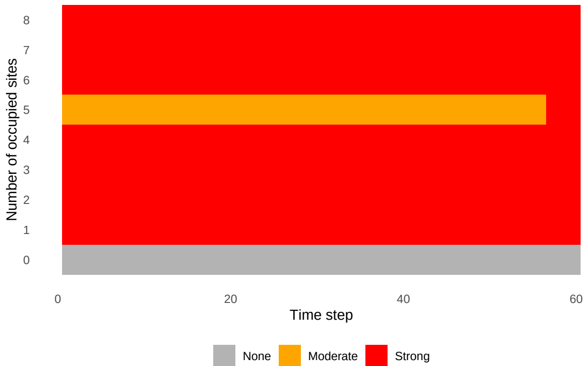
Figure 5: Optimal global action as a function of time and invasion level (measured as the number of occupied sites). Colors indicate the action recommended by the finite-horizon SDP (None/Moderate/Strong). This visualization highlights how stronger control becomes optimal as the invasion occupies more sites, and how recommendations may soften near the end of the planning horizon.
