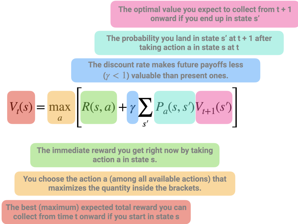
Figure 1: Representation of the Bellman equation in stochastic dynamic programming. The value of being in a given state at time t , V_t(s) , is defined as the maximum, over all possible actions, of two components: (i) the immediate reward obtained by taking action a in state s , and (ii) the expected discounted future value of subsequent states. The latter corresponds to the average (weighted by transition probabilities) of the optimal future values V_{t+1}(s') that can be reached from the current state-action pair, scaled by a discount factor \gamma < 1 to reflect that future payoffs are less valuable than present ones. This equation highlights the fact that the value of a decision is not only determined by its immediate payoff, but also by how it shapes future opportunities. The optimal action is therefore the one that maximizes the sum of current rewards and expected future benefits.
