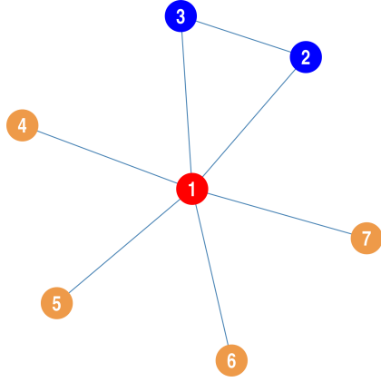
(c) Star Graph with Closure
