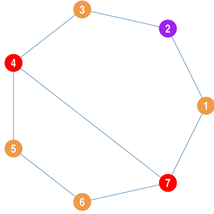
(b) Circle Graph with a Long Tie
