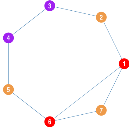
(a) Circle Graph with Closure
