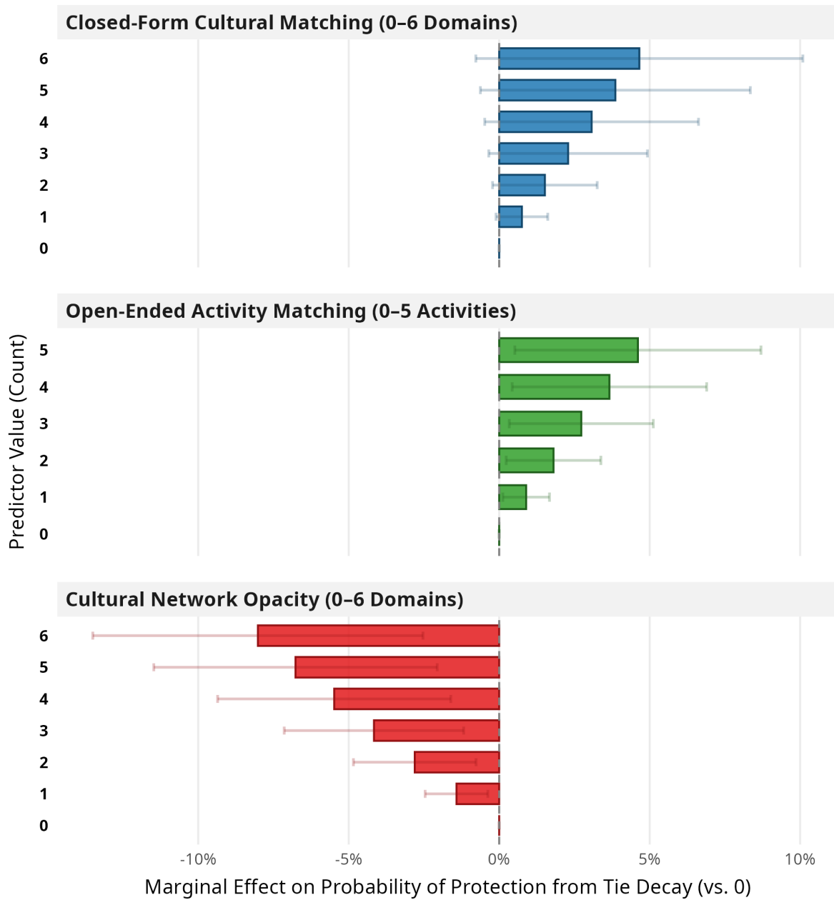
Figure 3: Within-Ego Marginal Effects on Protection from Tie Decay by Cultural Matching and Opacity Counts (Ego Fixed-Effects).
