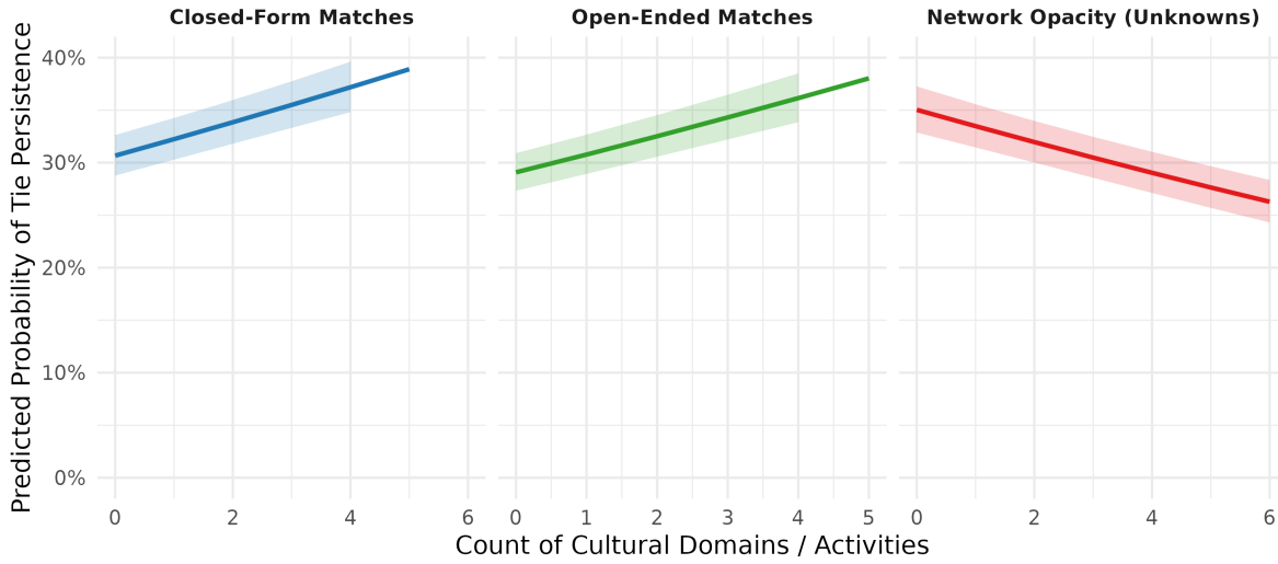
Figure 1: Predicted Probability of Tie Persistence by Cultural Matching and Cultural Network Opacity.
