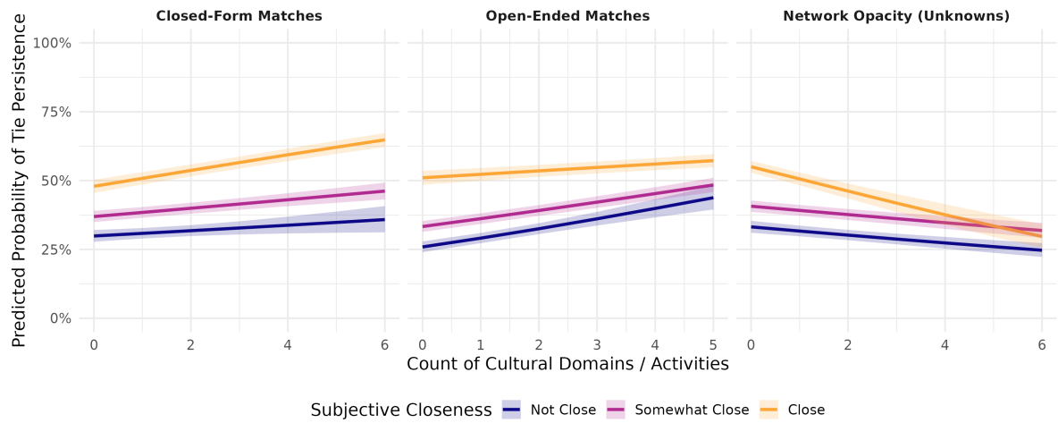
Figure 2: Predicted Probability of Tie Persistence by Cultural Matching, Cultural Network Opacity, and Subjective Closeness.
