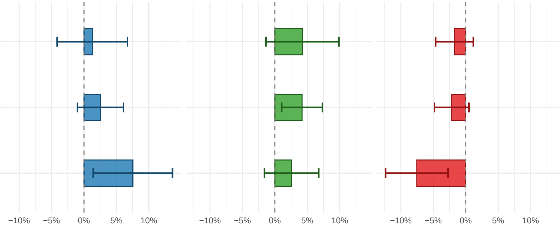
Closed-Form Matches
