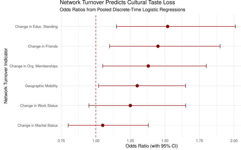
Figure 2: Network Turnover Predicts Cultural Taste Loss. Point estimates and 95% confidence intervals from pooled discrete-time logistic regressions.
