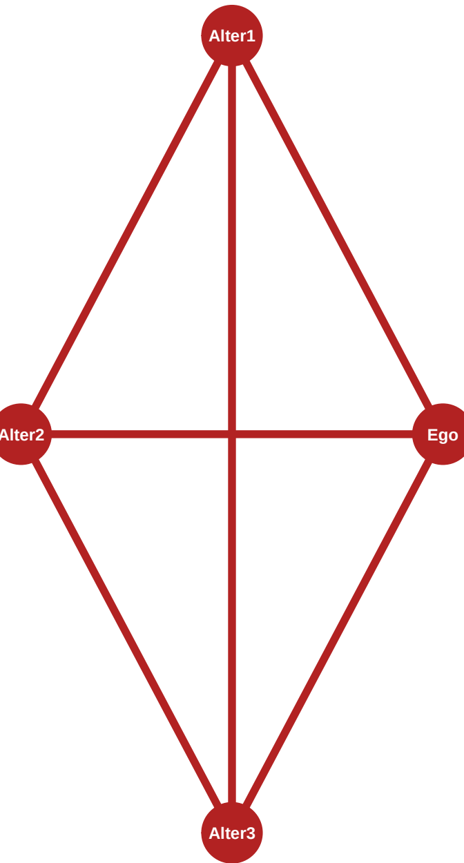
Clustered Network (Strong, High-Bandwidth Ties)
