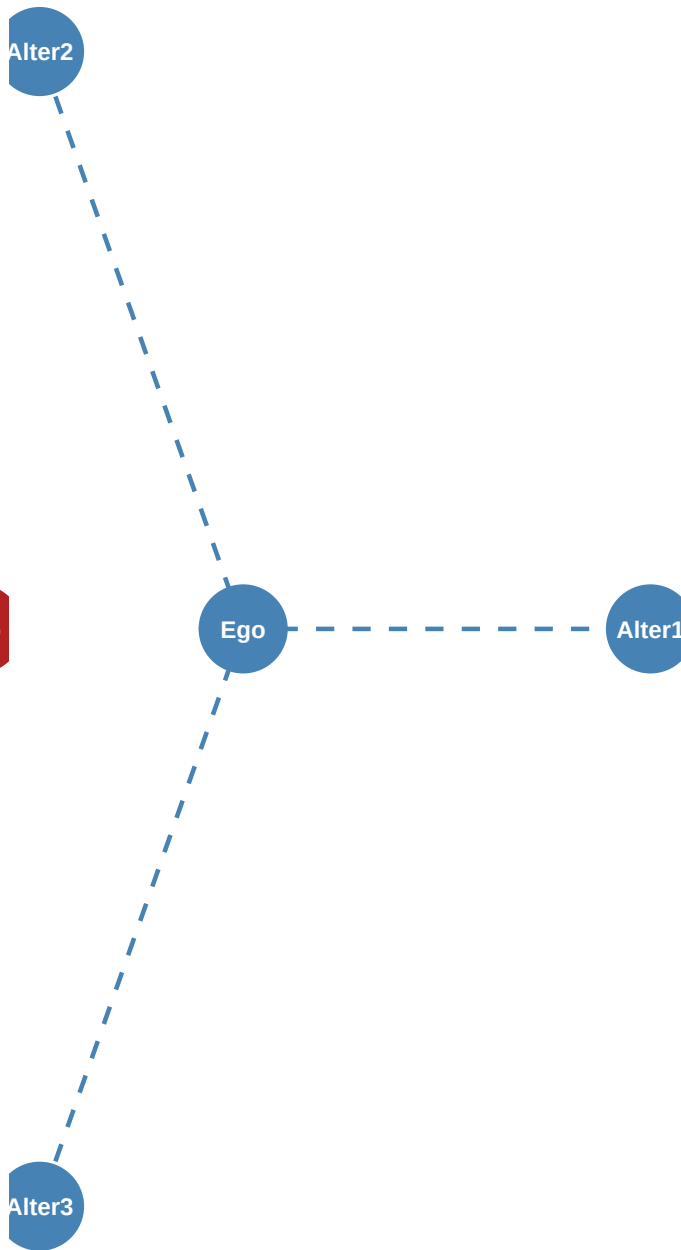
Unclassified Network (Weak, Low-Bandwidth Ties)
