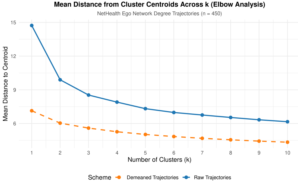
Figure 4: Mean Euclidean distance from cluster centroids across k = 1 \dots 10 cluster solutions for raw and demeaned degree sequences ( N = 450 ).
