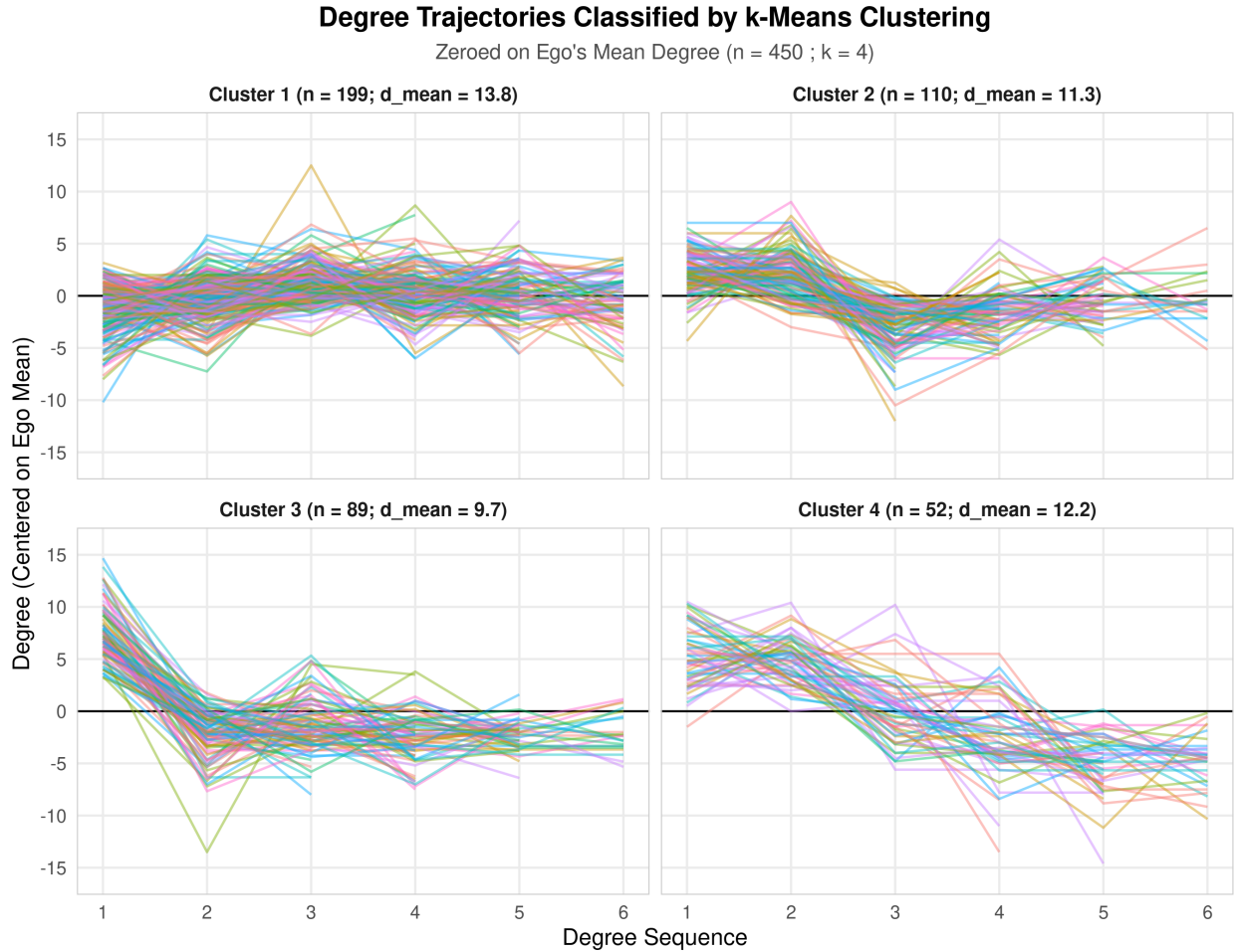
Figure 3: Degree trajectories classified by k -means clustering zeroed on ego mean ( k = 4 , N = 450 ). Trajectories represent deviations from each ego's longitudinal mean ( \tilde{D}_{it} = D_{it} - \bar{D}_i ).
