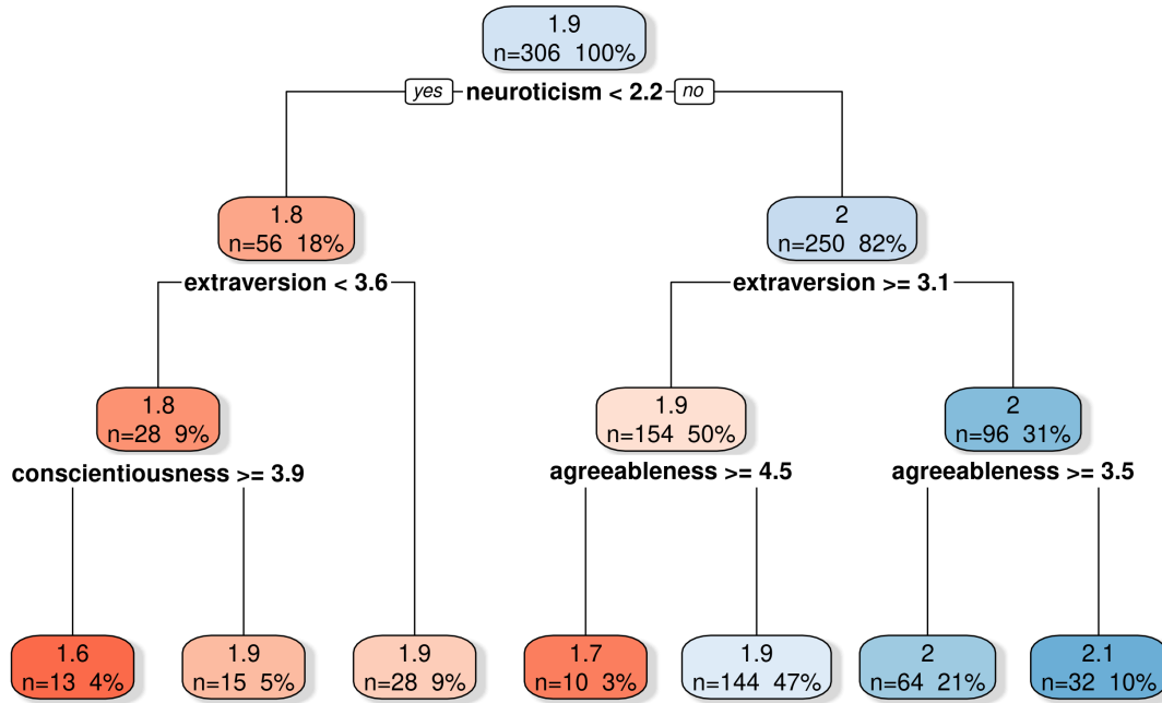
Figure S3: Classification and Regression Tree (CART) Predicting Social Signature Power-Law Alpha ( \alpha_i ) from Big Five Personality Traits ( N = 306 ). Node boxes display predicted mean \alpha_i (top) and sample size (bottom). Cross-validated error exceeds 1.0 at every split, indicating weak out-of-sample predictive value; the tree is reported as an exploratory, descriptive structure only. See main text Section 5.4.
