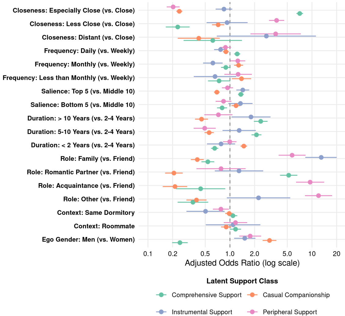
Figure 2: Adjusted Odds Ratios from Multilevel Logistic GLMMs Predicting Latent Social Support Configurations
