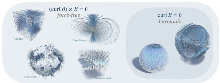
Fig. 2. Force-free fields emerge across fluid dynamics, plasma physics, and geometry. Their conformal geodesibility connects these settings, identifying field lines with geodesics of a rescaled metric [P2].
