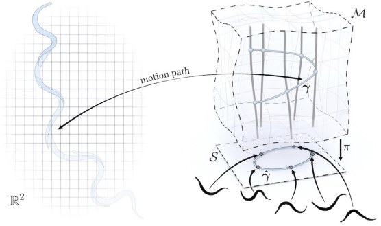
Fig. 5. In geometric models of locomotion, gauge connections reconstruct a snake's motion from its path through shape space [35].
