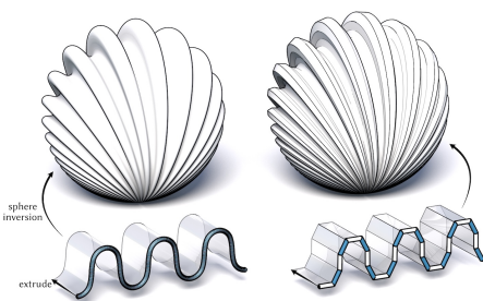
Fig. 9. Willmore surfaces obtained from analogous continuous (left) and semi-discrete (right) constructions.
