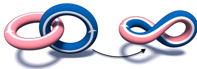
Fig. 4. Reconnection converts mutual linking into flux-tube twist.
