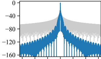
(a) Cosine
