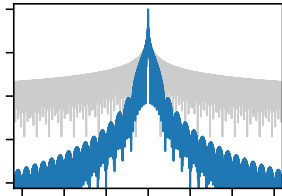
(b) Hann
