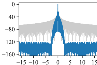
(c) Blackman
