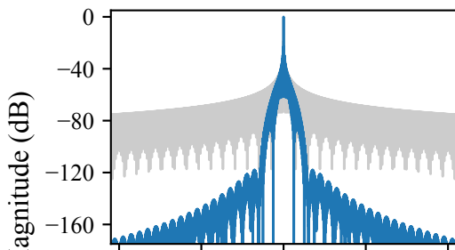
(c) Blackman
