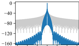
(c) Blackman
