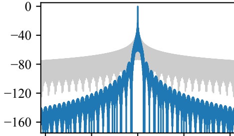
(a) Cosine
