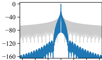
(c) Blackman
