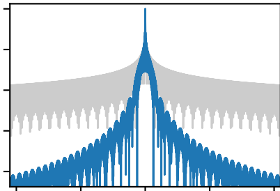
(b) Hann
