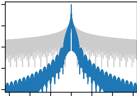
(b) Hann
