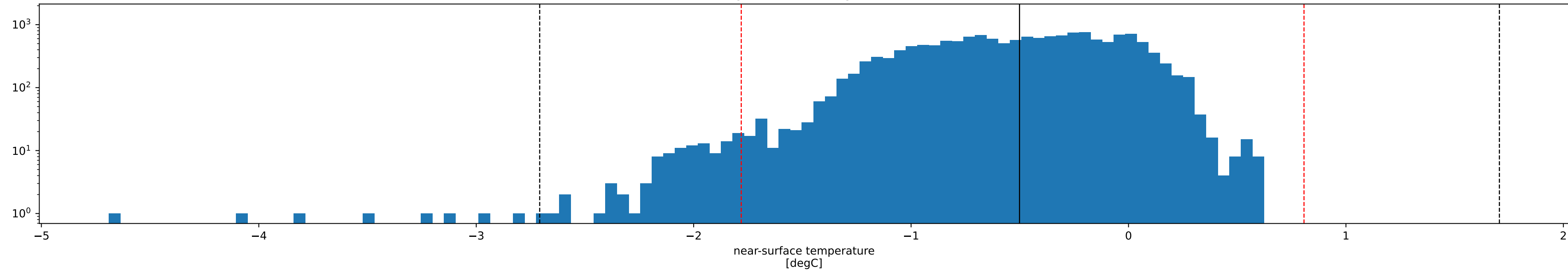
Filtered variance log10 tas
