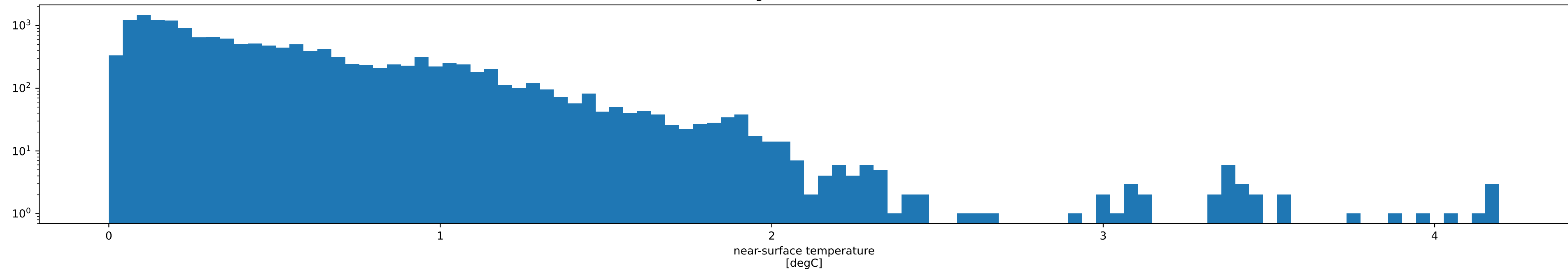
Original variance log10 tas
