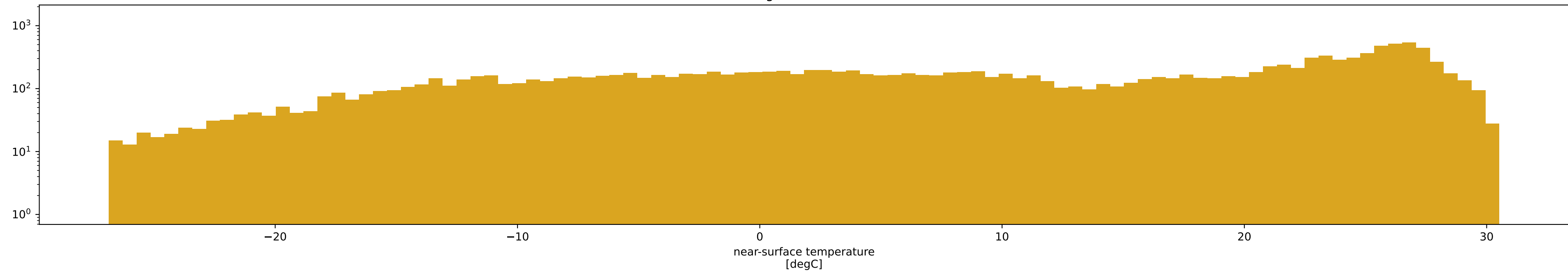
Original variance tas
