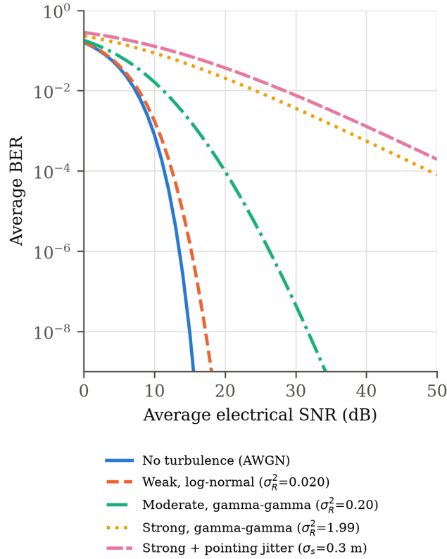
Fig. 7. Average BER of OOK IM/DD at 1550 nm over 1 km for log-normal and gamma-gamma turbulence, with and without pointing jitter. A point receiver is assumed, so aperture averaging is not included.
