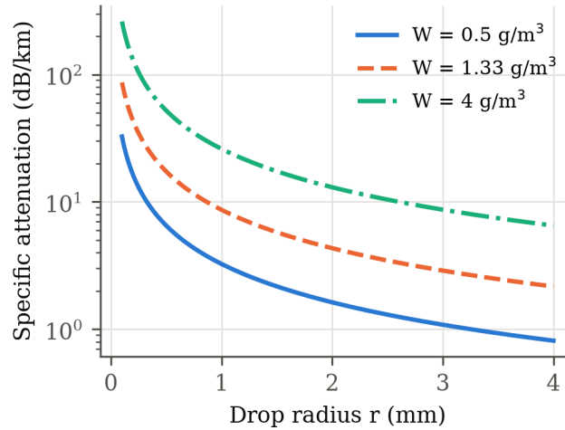
Fig. 4. Specific attenuation of monodisperse large drops versus drop radius at fixed liquid water content W , from (12) with Q_{ext} = 2 . The value 1.33 \text{ g/m}^3 corresponds to Marshall–Palmer rain at 25 \text{ mm/h} .
