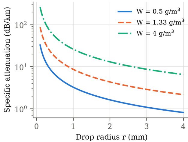
Fig. 4. Specific attenuation of monodisperse large drops versus drop radius at fixed liquid water content W , from (12) with Q_{ext} = 2 . The value 1.33 g/m 3 corresponds to Marshall–Palmer rain at 25 mm/h.
