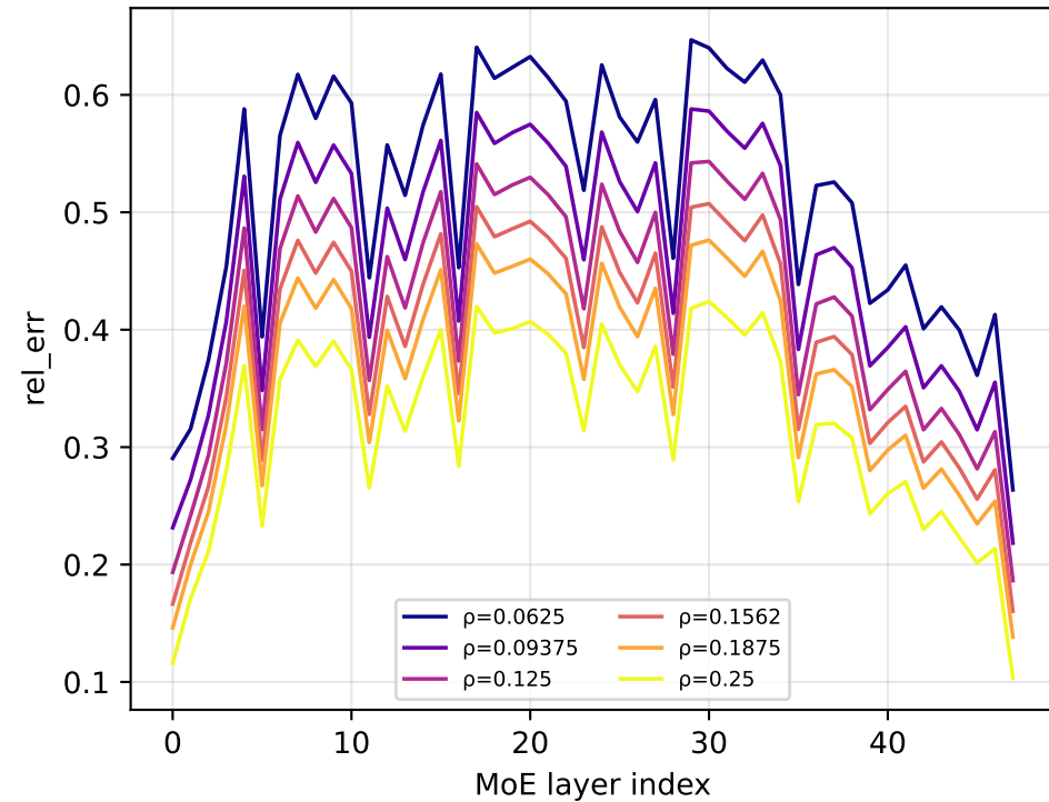
Layers are not interchangeable ( p=0.25 ) at p=0.125 : min 0.186, max 0.543 ( 2.92\times )
