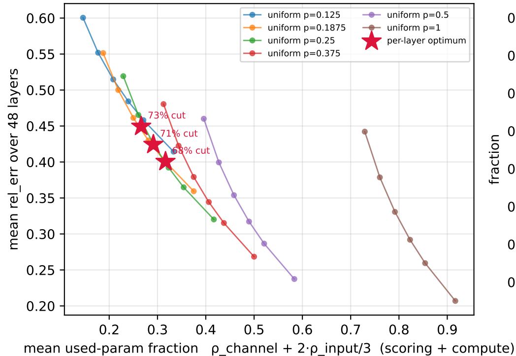
Per-layer allocation vs the uniform frontier (stars: slope-weighted solve, scored on unweighted err)
