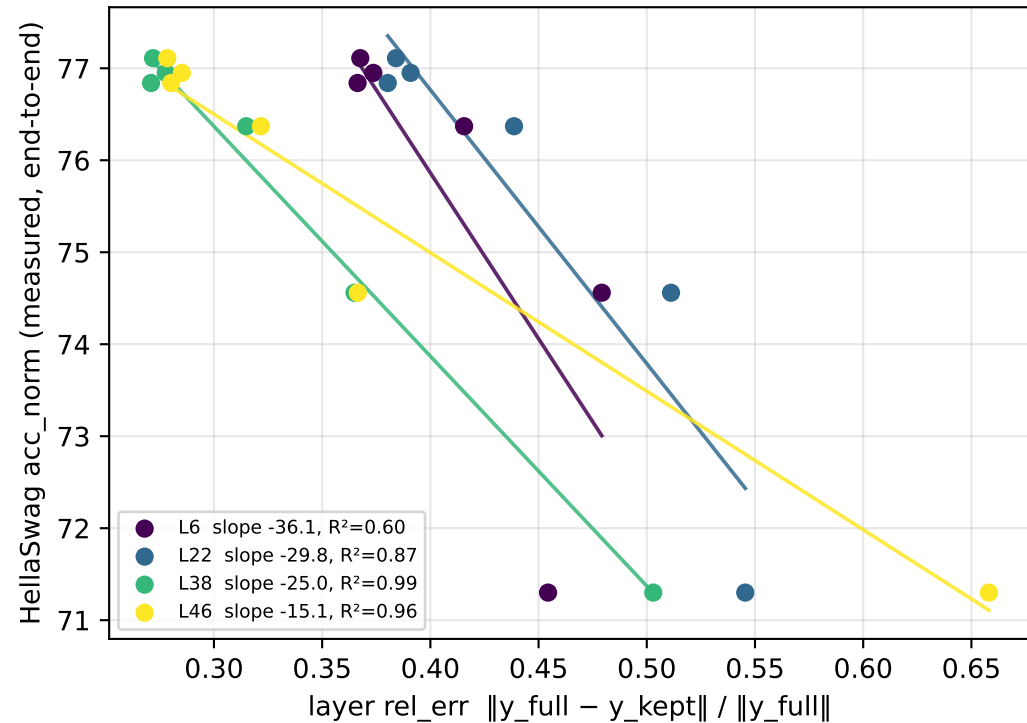
Per-layer rel_err vs final accuracy (fixed budget \rho=0.125 , selector varying)
