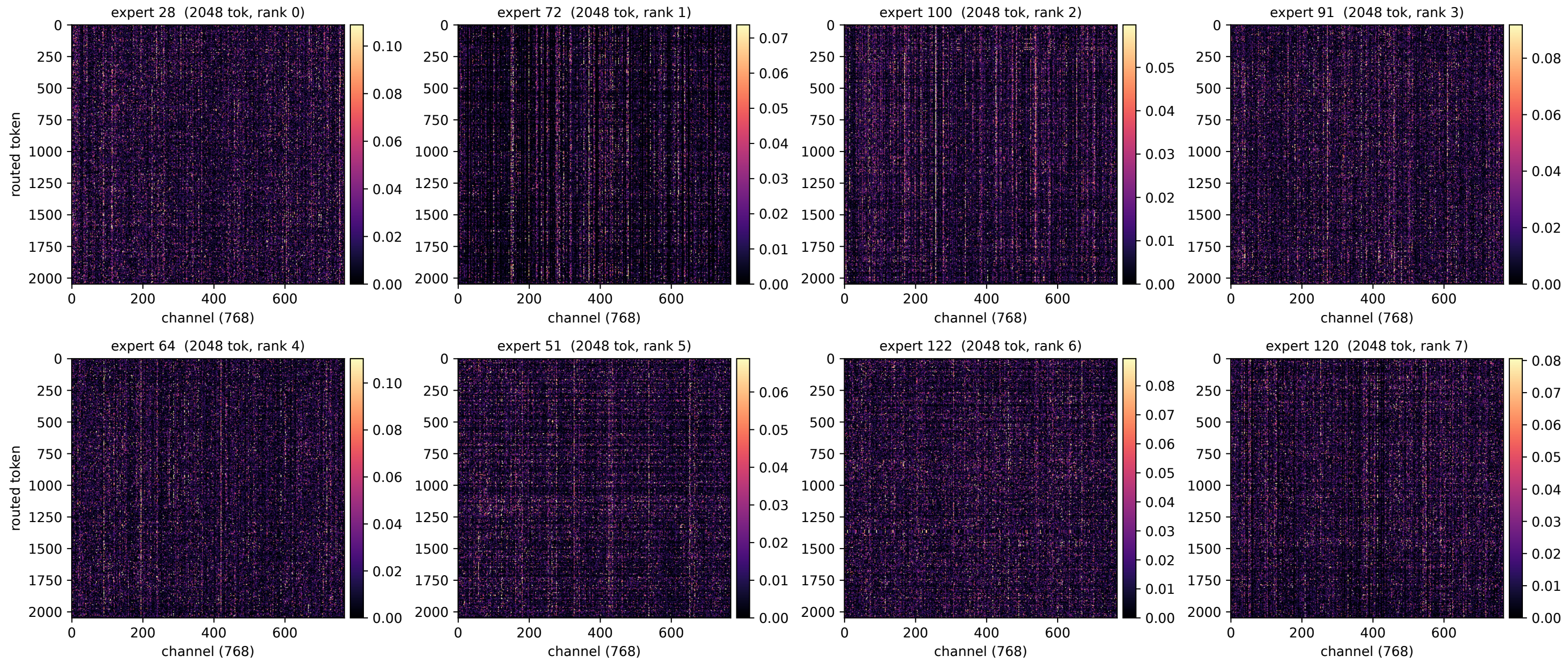
Layer 0: per-expert intermediate |SwiGLU| (input of down_proj), top-8 most-routed experts [128/128 experts used]
