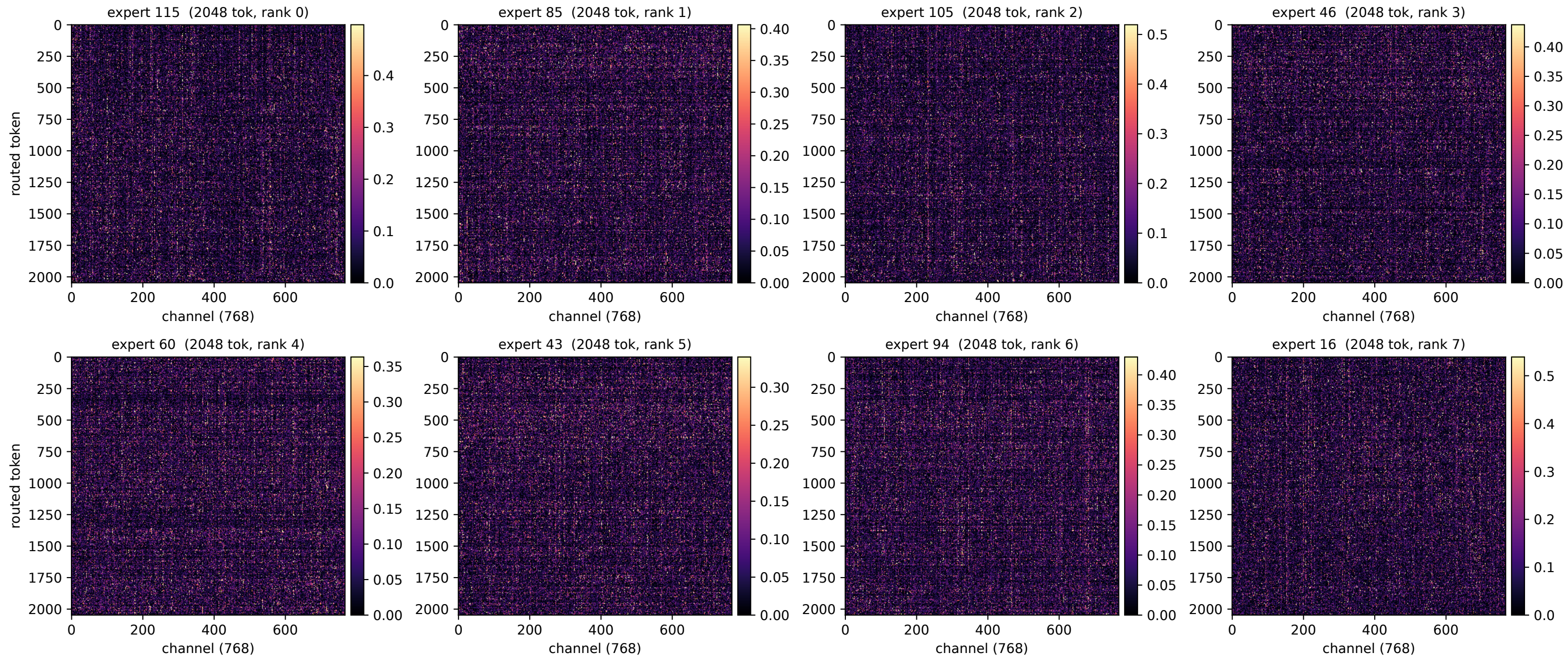
Layer 11: per-expert intermediate |SwiGLU| (input of down_proj), top-8 most-routed experts [125/128 experts used]
