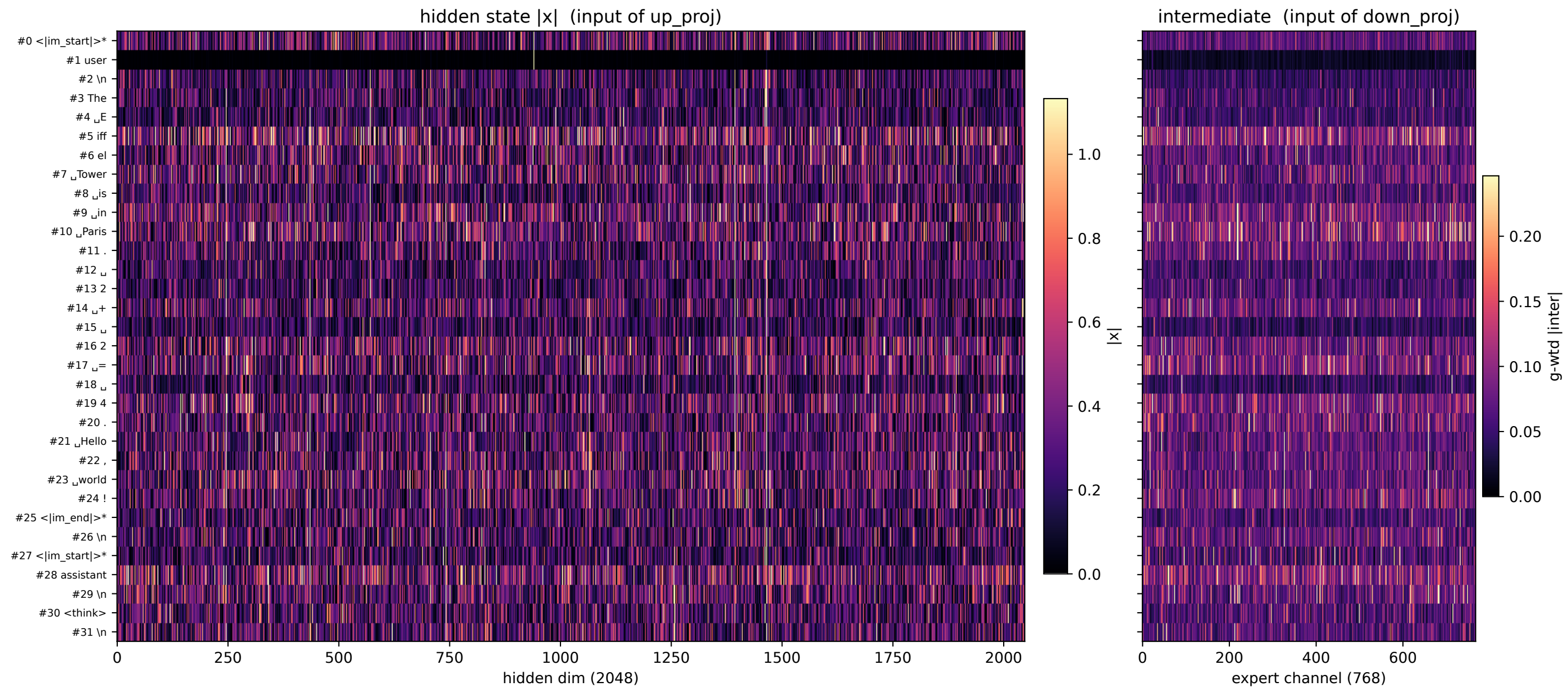
Layer 11: hidden state & intermediate across the 32 prompt tokens (* = special token)
