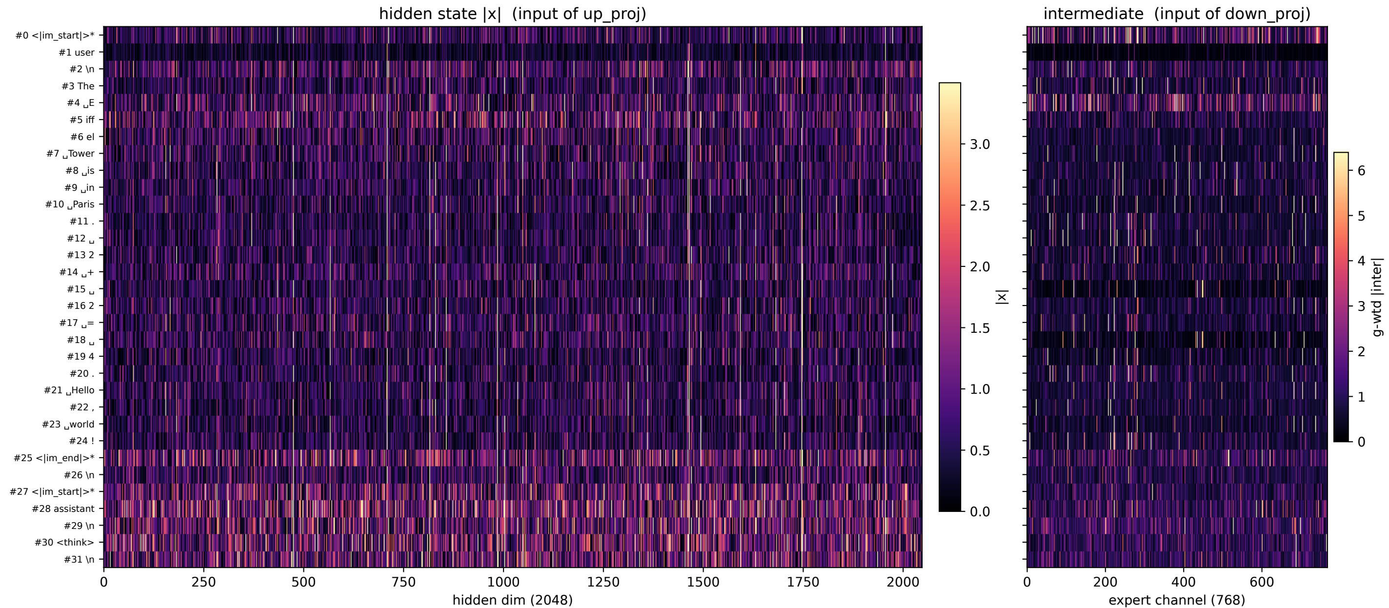
Layer 47: hidden state & intermediate across the 32 prompt tokens (* = special token)
