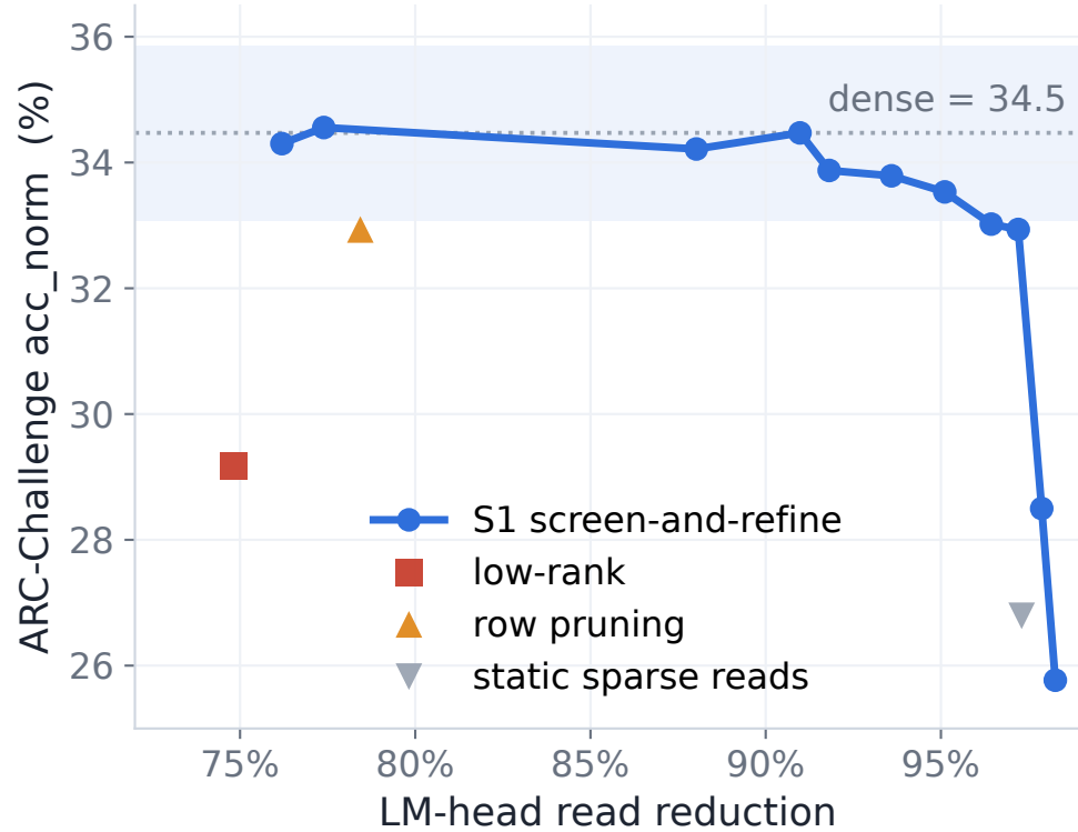
ARC-Challenge vs how much of the lm_head a token can skip
