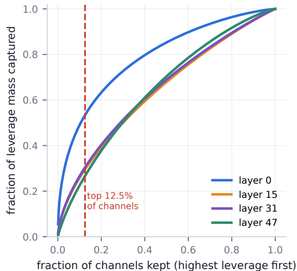
(b) ...so most of the mass is in a small prefix
