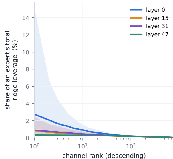
(a) Early layers: a few channels carry it
