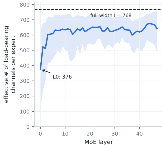
(c) Early layers compress most
