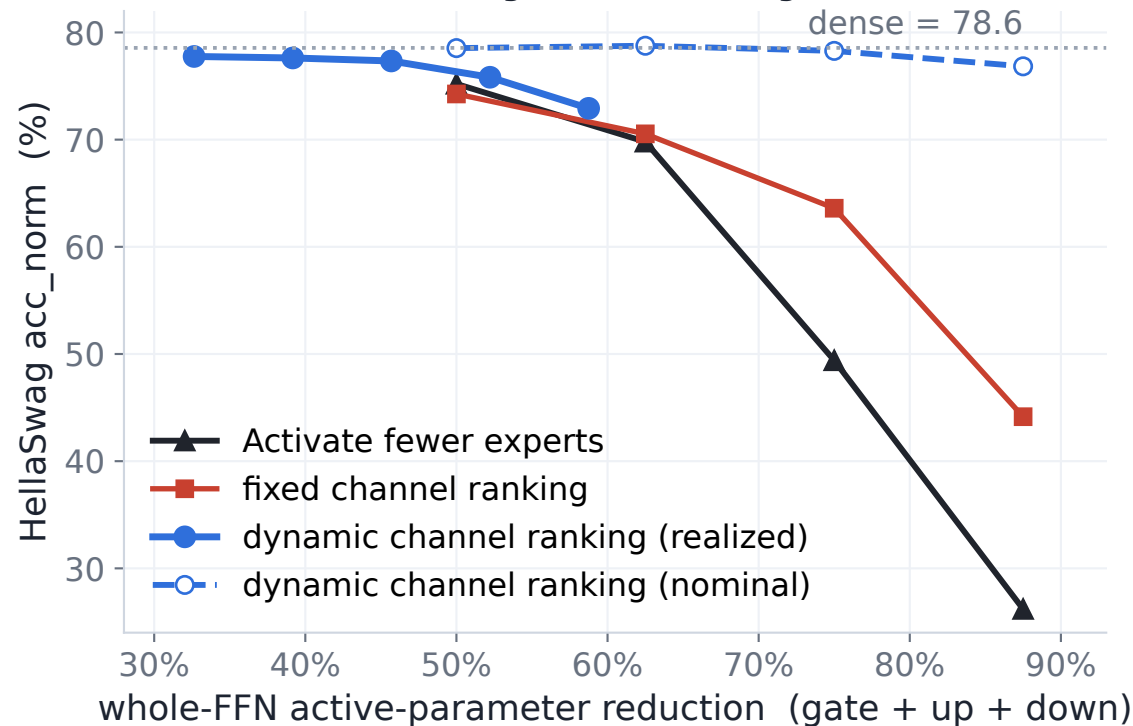
Online per-token selection stays near dense where offline collapses Qwen3-30B-A3B-Thinking-2507, HellaSwag 0-shot, no fine-tuning
