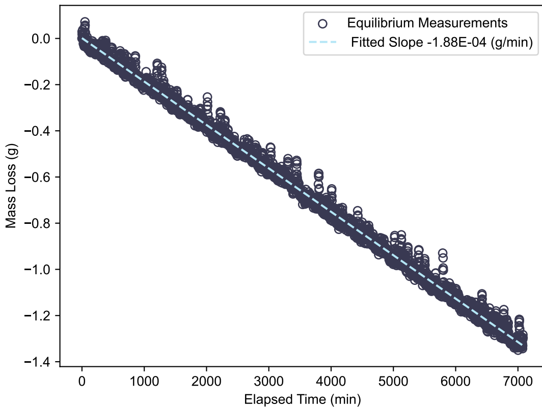
Cellulose_10
