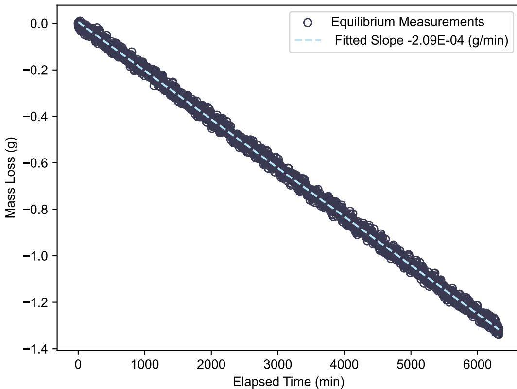
Cellulose_1
