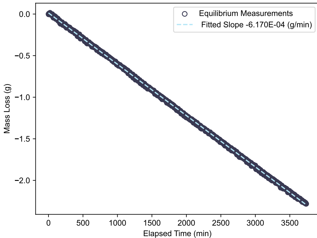
Marino-wool_1
