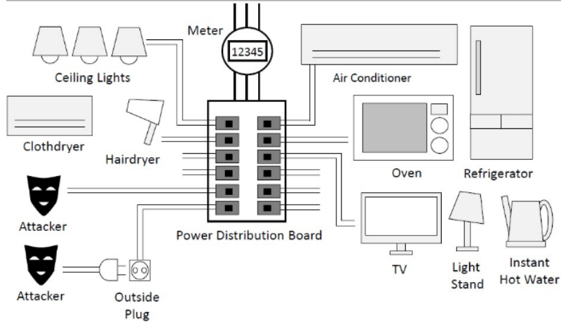
Fig. 1: Scenarios of electricity theft attacks in this study. Power distribution boards and cables are deployed behind walls and are usually not visible. An attacker uses the pre-deployed cable in a complex building or the outside plug to steal electricity. Depending on the theft pattern, we identify five classes of attacks.
